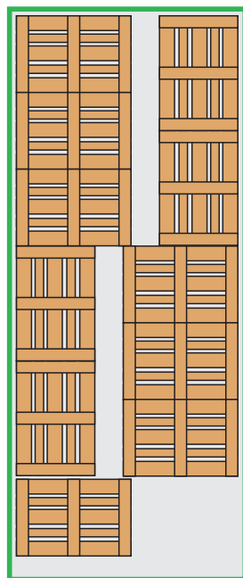
20' STANDARD 11 EUR pallets
